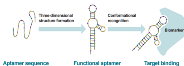
Figure 2: Aptamer formation
