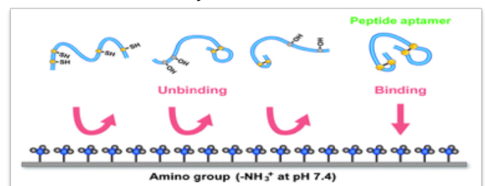
Figure 8: Amino group binding peptide aptamers with double disulphide-bridged loops
