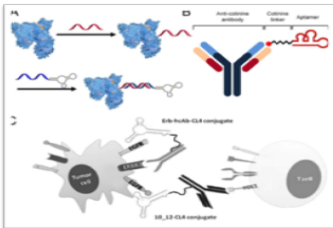
Figure 3: Aptamer-Drug Conjugate
