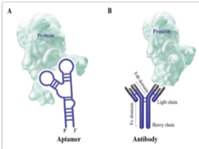
Figure 6: Difference between Aptamer and Antibody
