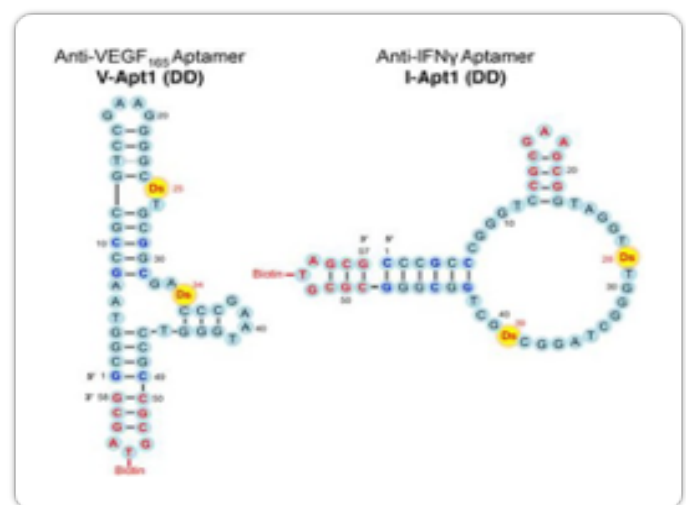
Figure 4: Aptamers
