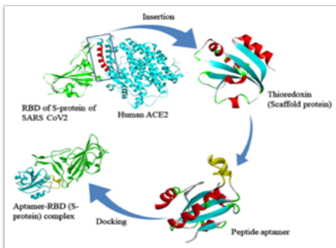
Figure 7: Designing of peptide aptamer targeting the receptor-binding domain of spike protein of SARS-CoV-2
