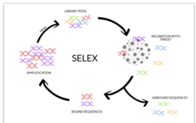
Figure 5: SELEX Cycle
