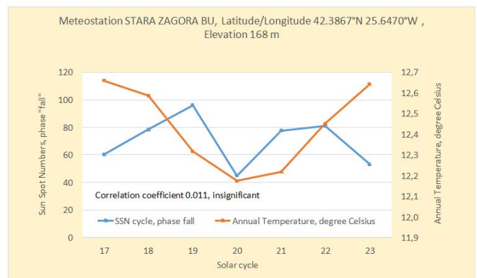
Figure 3: There is no statistically significant correlation between the mean surface air temperature for the weather station STARA ZAGORA, BULGARIA, and the mean number of sunspots during the phase “fall” of the last 7 cycles of solar activity.
