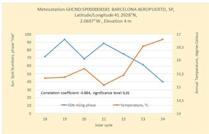
Figure 10: There is a high statistically significant negative correlation between the mean surface air temperature for weather station BARCELONA AEROPUERTO, SPAIN, and the mean sunspot number during the phase “rise” of the 7 cycles of solar activity (for which data are available).
