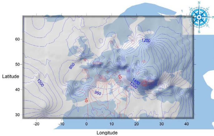
Figure 14: The main areas of influence of solar alpha radiation on mortality in the Europe and Mediterranean region are the Balkans and, to a lesser extent, the Western Mediterranean. (Software Surfer 10).
