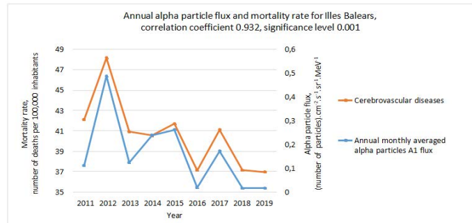
Figure 15: There is a high statistically significant correlation between the annual flux of highenergy solar alpha particles and cerebrovascular disease mortality in the Western Mediterranean, i.e. it is very likely that there is a causal relationship between the two phenomena.
