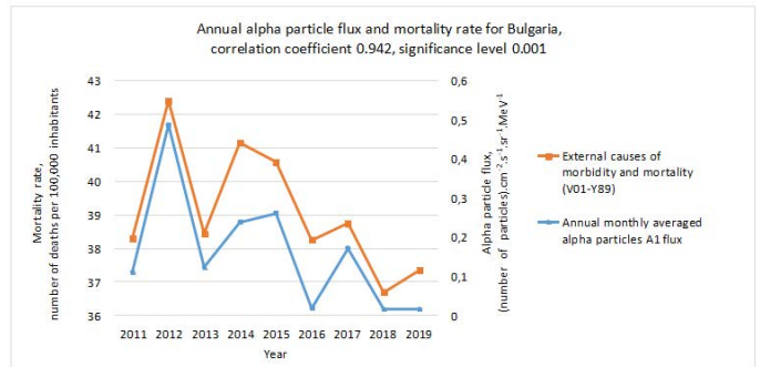
Figure 17: There is a high statistically significant correlation between the annual flux of solar alpha particles with high energy and the mortality from external causes of death in Bulgaria, i.e. it is very likely that there is a causal relationship between the two phenomena.
