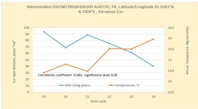
Figure 9: There is a high statistically significant negative correlation between the mean surface air temperature for weather station AJACCIO, FRANCE, and the mean sunspot number during the phase “rise” of the 6 solar activity cycles (for which data are available).
