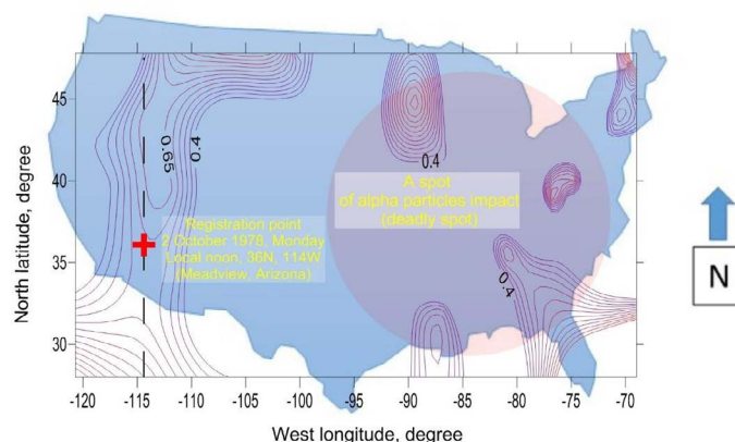
Figure 18: Alpha radiation flux registration point (red cross) from October 2nd, 1978, in the western USA, and the dead spot in the eastern US, tentatively denoted by a circle centered 30^\circ eastward from the registration point.
