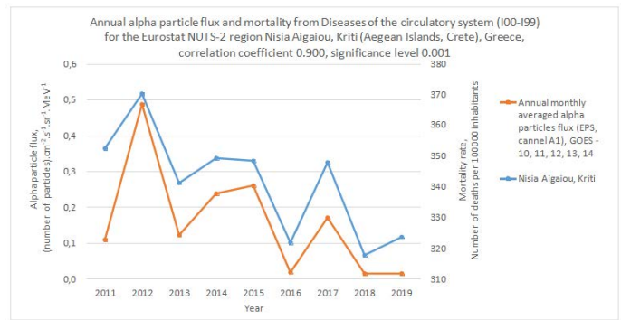
Figure 16: Between the annual flux of high-energy solar alpha particles and mortality from circulatory system diseases in the Aegean Islands and Crete, Greece, there is a high statistically significant correlation, i.e. it is very likely that there is a causal relationship between the two phenomena.
