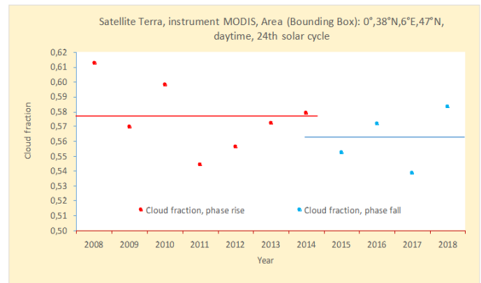
Figure 13: Daytime cloudiness over the western Mediterranean is about 1.5% more during the phase "rise" of the solar cycle than during the phase "fall".
