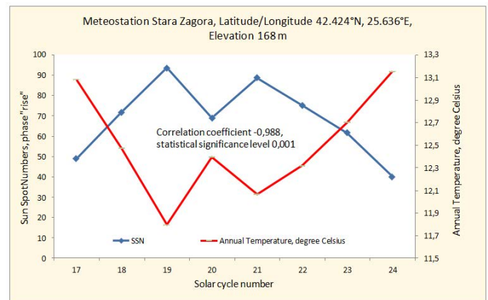
Figure 2: There is a high statistically significant negative correlation between the mean surface air temperature for the weather station STARA ZAGORA, BULGARIA, and the mean value of the number of sunspots during the phases “rise” of the last 8 cycles of solar activity.
