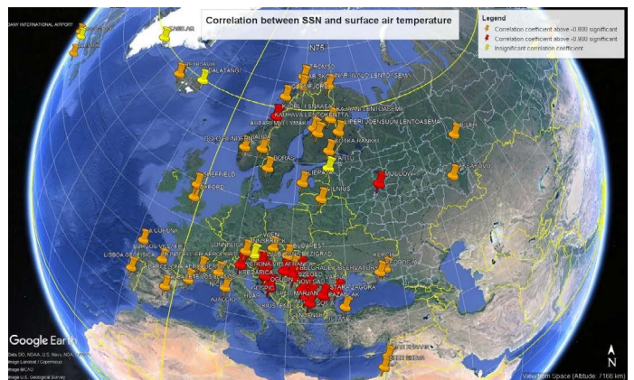
Figure 12: Google Earth map with stations from the Northern Hemisphere, the markers for which are colored depending on the magnitude of the correlation coefficient between surface air temperature and SSN for the phase “rise” of the solar cycles.
