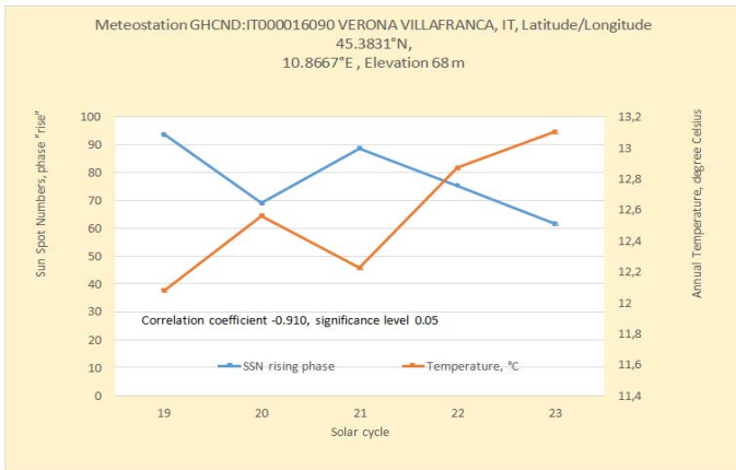
Figure 8: There is a high statistically significant negative correlation between the mean surface air temperature for weather station VERONA VILLAFRANCA, ITALY, and the mean sunspot number during the phase “rise” of the 5 cycles of solar activity (for which data are available).
