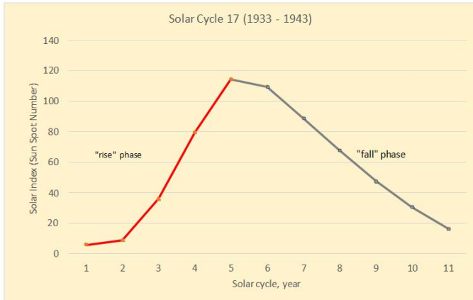
Figure 1: A cycle of solar activity in the example of solar cycle 17 (chosen for its good shape). During the first phase of the cycle, solar activity increases, and reaches a maximum (the largest number of sunspots), then during the second phase, the activity decreases to a minimum before the start of the next cycle.
