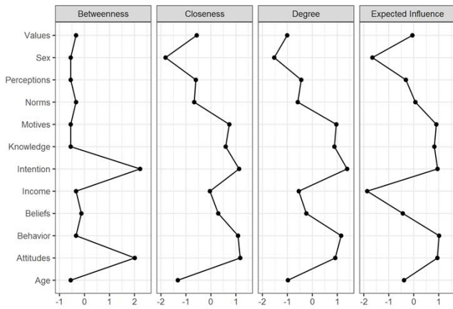
Figure 1: Eigenvalues
